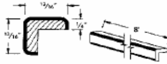
Outside Corner Scribe (OCS)
